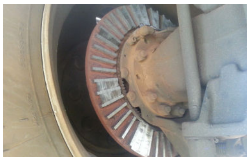
Worn Rotor. OOSC, Part II, g.(3) / 393.47(g) -U.S.
